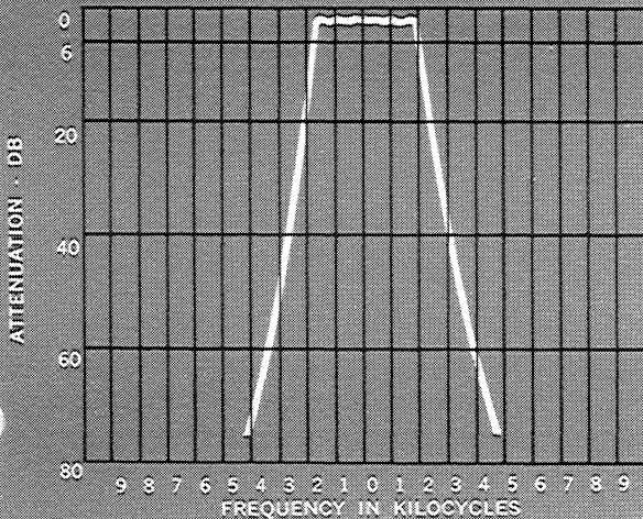
F455-40 Center frequency 455 kc; 6 db bandwidth 4.0 kc; 60 db bandwidth 8.5 kc maximum.
